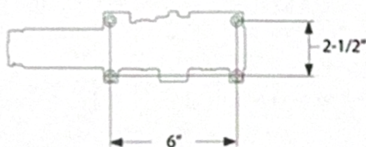
2-1/2" Vertical Holes x 6" Horizontal Holes LCN 4011, 4021, 4111
