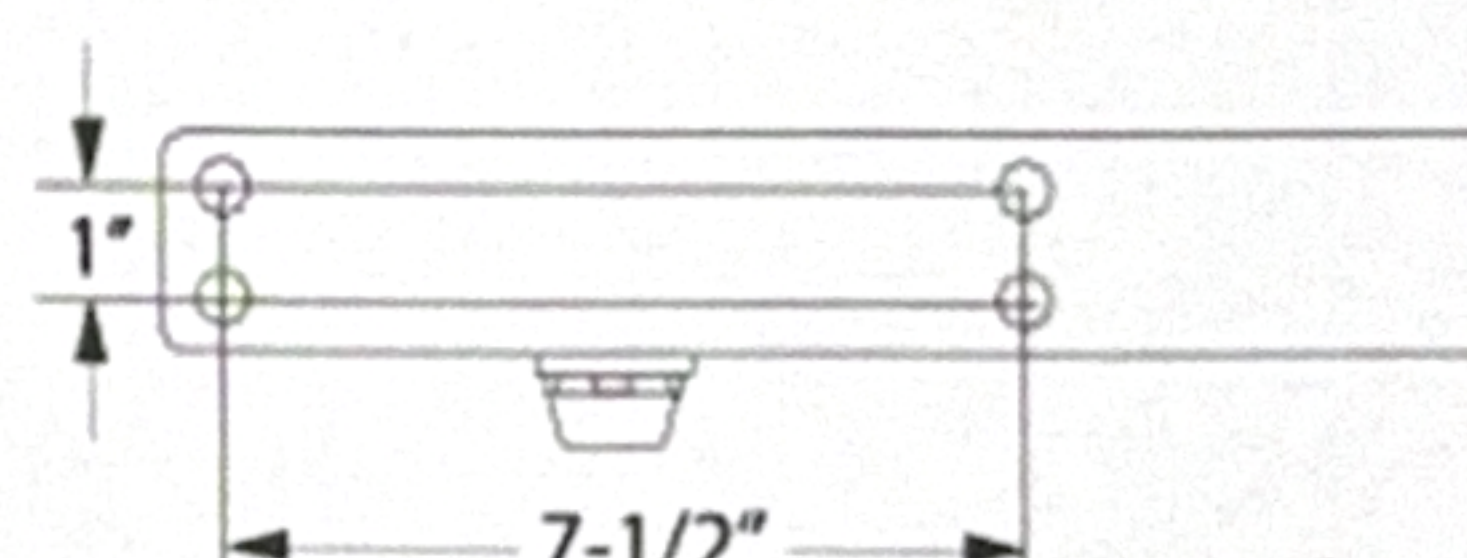
1" Vertical Holes x 7-1/2" Horizontal Holes LCN 1461
