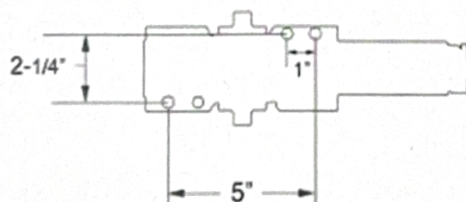
2-1/4" Vertical Holes x 5" Horizontal Holes Trudoor TDC-400 LCN 4040XP Yale 5800 Hager 5100 Cal-Royal CR441 Design Hardware 416 Stanley QDC-111
