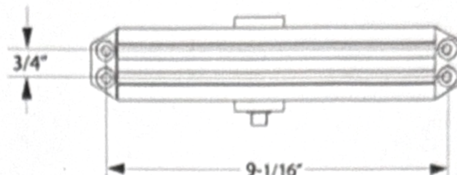
3/4" Vertical Holes x 9-1/16" Horizontal Holes
